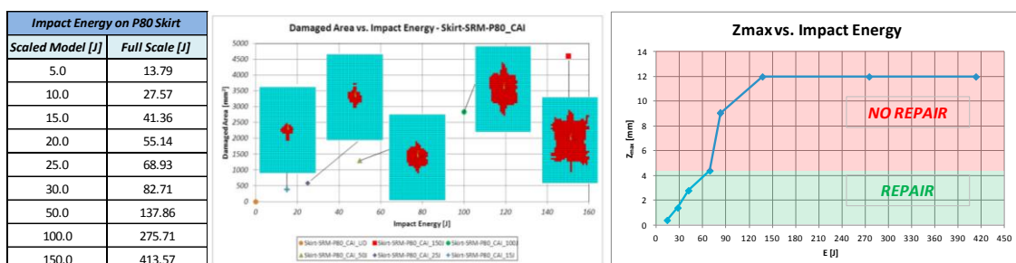
Figure 2. Relation between scaled and full-scale impact energy. Damaged Area on scaled thickness flat panel. Damage depth on full thickness flat panel.
