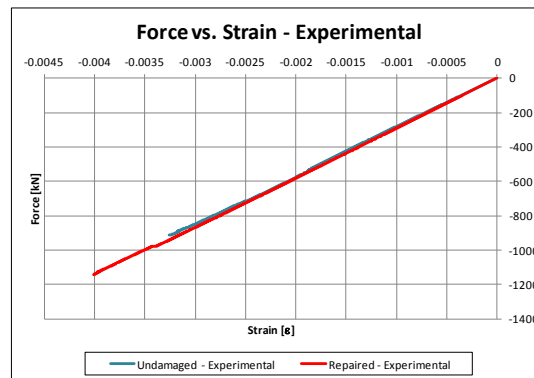
Figure 14. experimental compression test: load vs. applied strain curve
