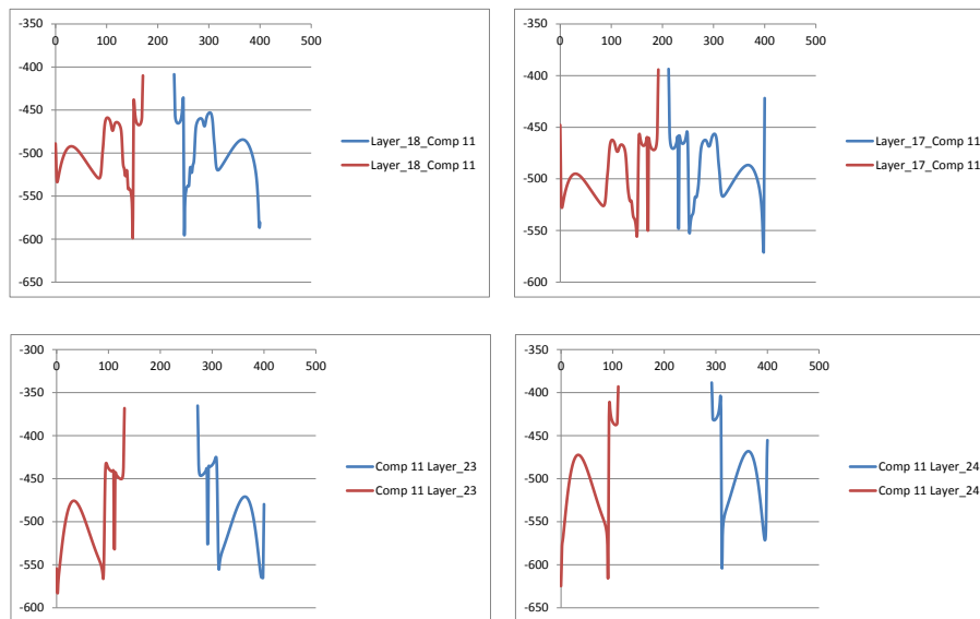
Figure 12. \sigma_{11} stress [MPa] in 0^\circ original plies
