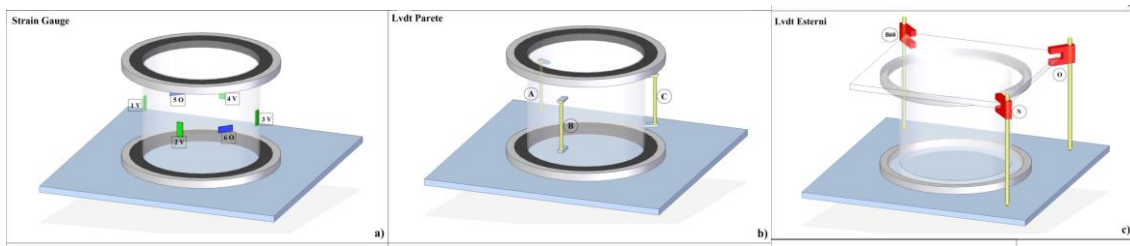
Figure 13. Strain gauges and LVDT locations
