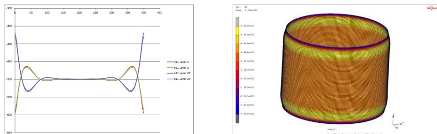
Figure 10. \sigma_{11} in inner and outer 0^\circ ply and failure elements at 1140 kN
