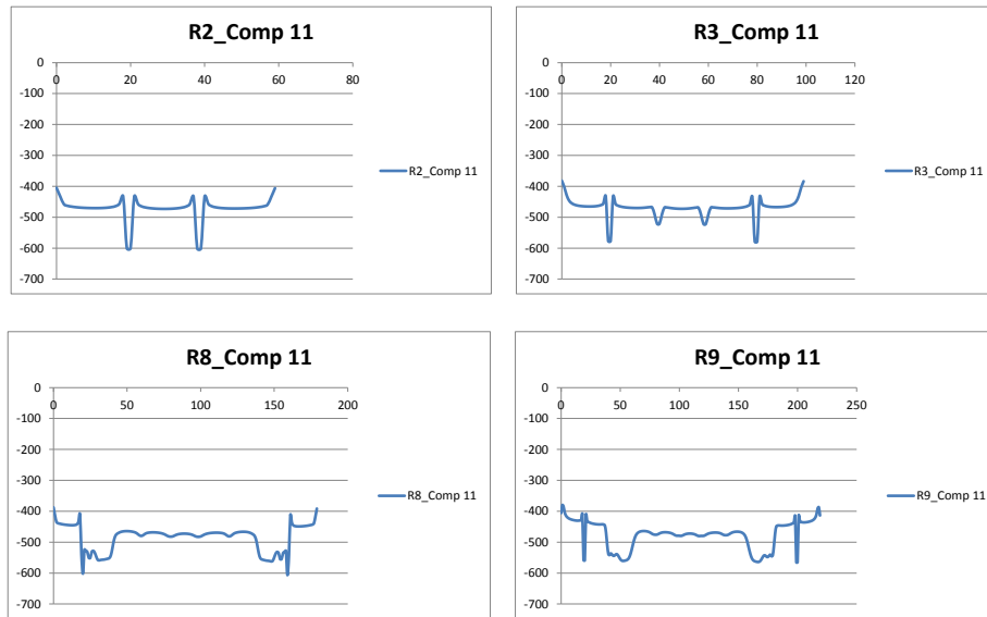
Figure 11. \sigma_{11} stress [MPa] in 0^\circ Repair laminas
