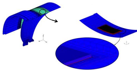
Figure 4. Global-Local models used for the numerical analysis
