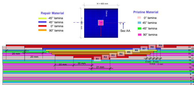
Figure 5. Repair scheme
