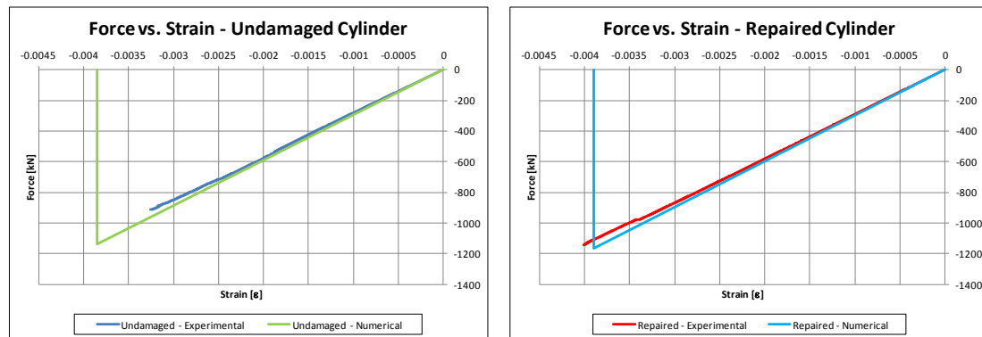
Figure 17. Comparison between numerical and experimental results
