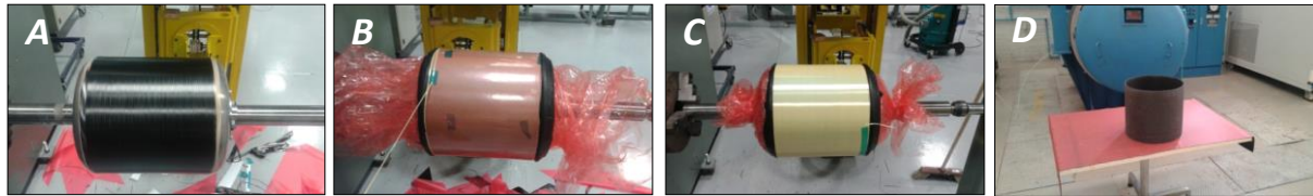
Figure 7. Filament winding of the hoop layers (A), Release film (B) and Kevlar winding (C), Undamaged Cylinder (D)
