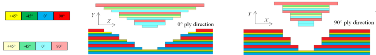
Figure 3. P80 Skirt repair schema
