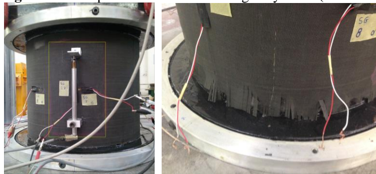
Figure 16. Compression Test of repaired cylinder
