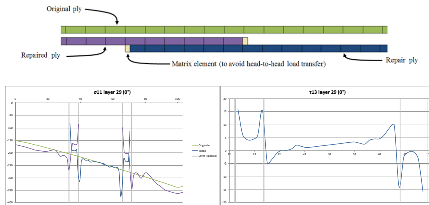
Figure 6. Fiber load and interface shear stress distribution for the most critical layer in the P80 SRM repaired skirt
