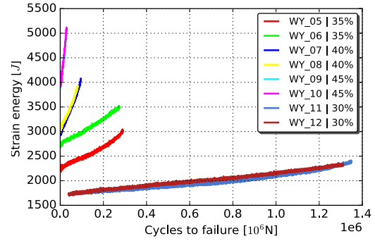
Figure 5: Strain energy vs cycles to failure.
