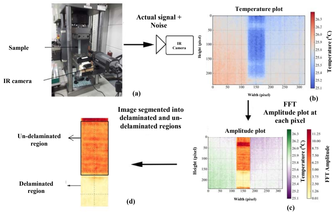
Figure 2: Block diagram of the processing algorithm a) Sample in test frame, b) Temperature plots obtained from IR camera, c) FFT amplitude plot and d) Image segmented image with delaminated and un-delaminated area.
