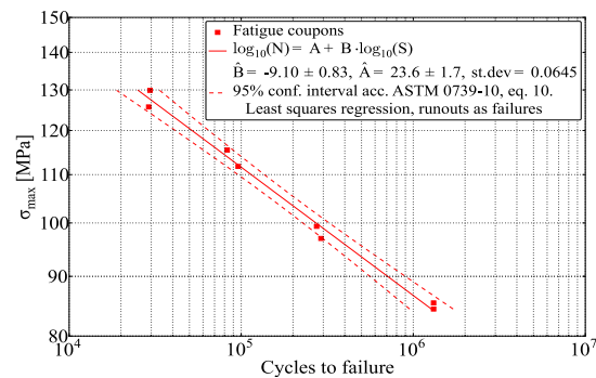
Figure 7: S-N curves with least square fit.
