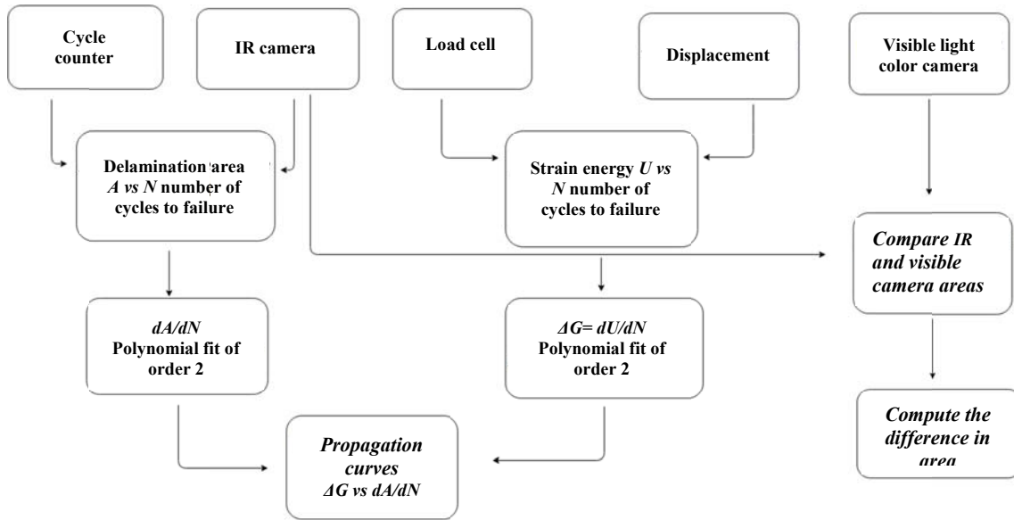
Figure 3: Test process flow to arrive at fatigue growth curves.
