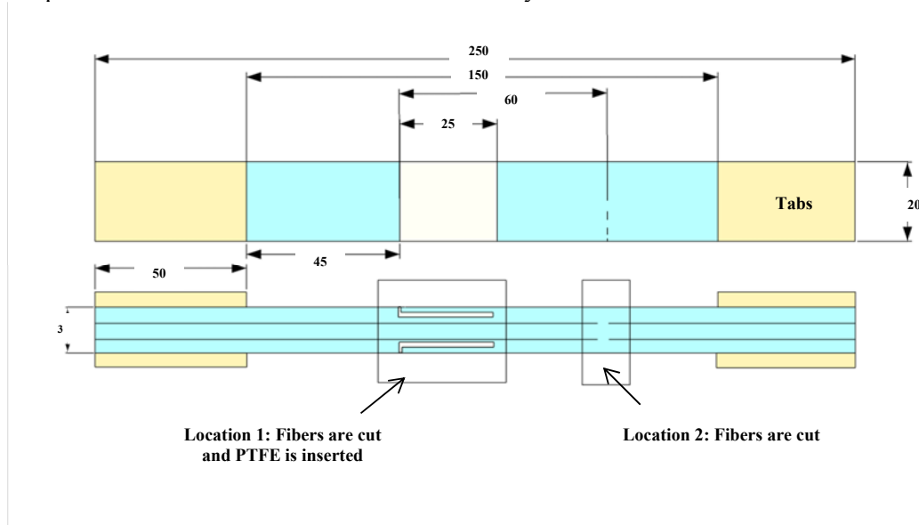
Figure 1: Diagram of the double shear configuration coupon. All dimensions are in mm.
