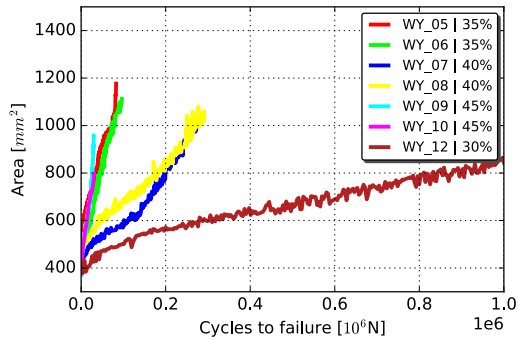
Figure 4: Area vs cycles to failure A(N) .
