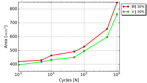
Figure 8: Comparison of measurement by the IR camera and visible camera.
