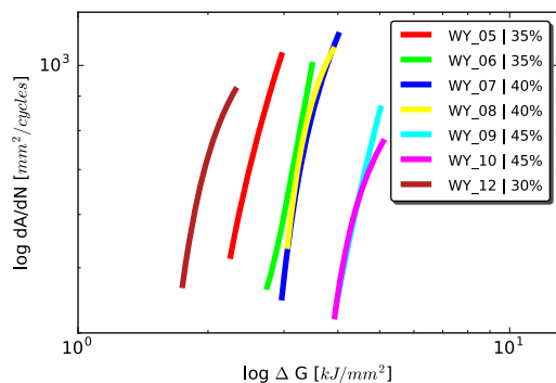
Figure 6: Propagation curves (dA/dN vs \Delta G) .
