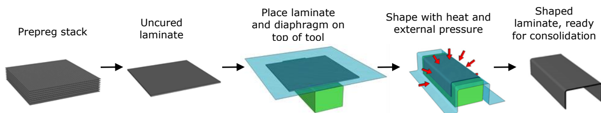
Figure 1. Illustration of composite vacuum forming process.
