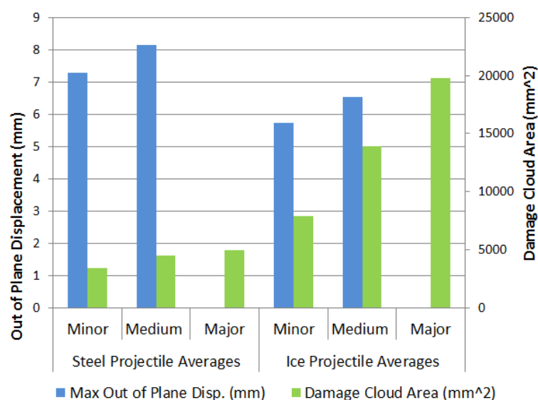
Figure 4. Maximum out-of-plane displacements and damage areas for both solid steel and fragmenting ice projectiles
