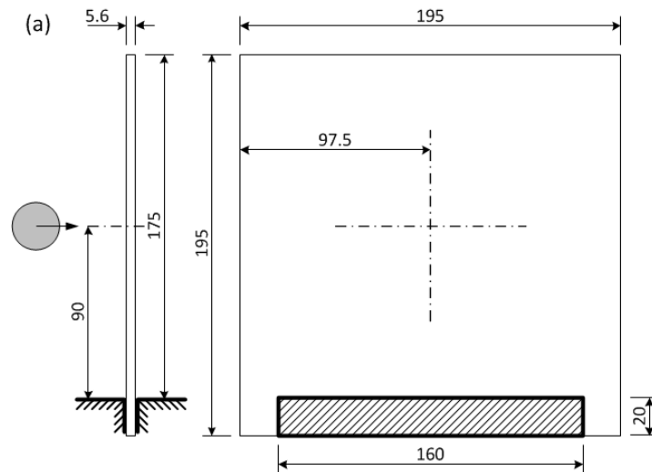
Figure 1. Ballistic impact regime and cantilever clamping fixture
