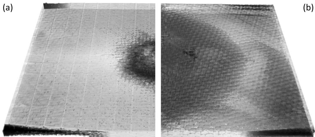
Figure 3. Typical examples of internal damage cloud in composite specimens caused by solid steel (a) and fragmenting ice (b) projectiles
