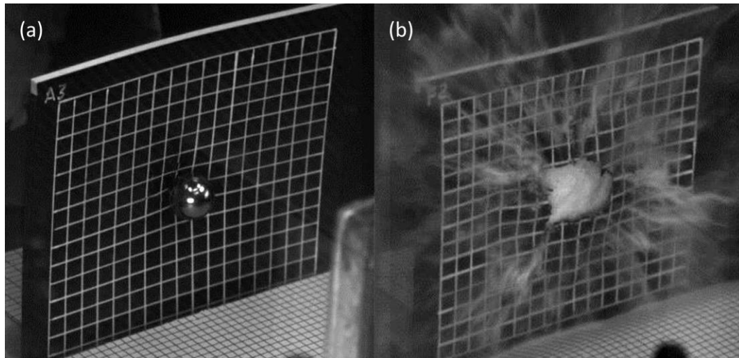
Figure 2. Typical impact behaviour of solid steel projectile at 0.40 ms (a) and fragmenting ice projectile at 0.19 ms (b)
