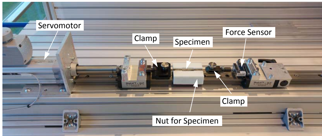
Figure 4. Lap shear test stand
