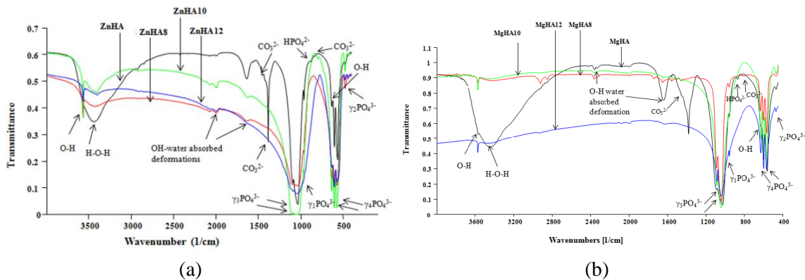
Figure 3. FTIR Spectra of as-synthesized and calcined (a) ZnHA (b) MgHA nanopowders.
