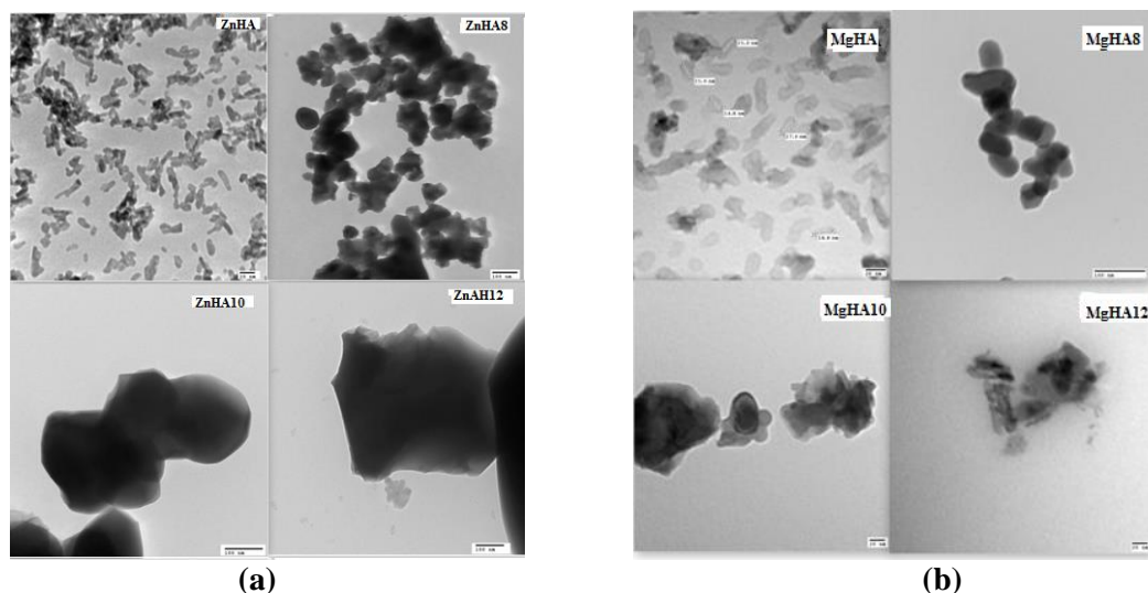
Figure 1. TEM micrographs of as-synthesized and calcined (a) ZnHA (b) MgHA nanopowders.
