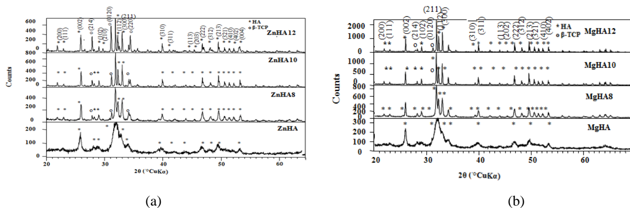
Figure 2. XRD patterns of as-synthesized and calcined (a) ZnHA (b) MgHA nanopowders.
