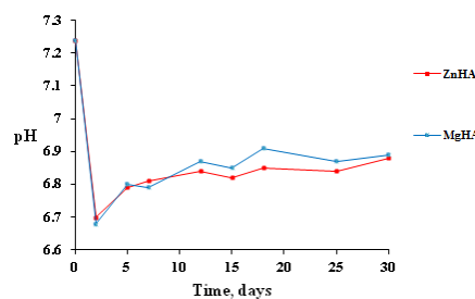
Figure 4. pH change in SBF with time of immersion for as-synthesized ZnHA and MgHA nanopowders.
