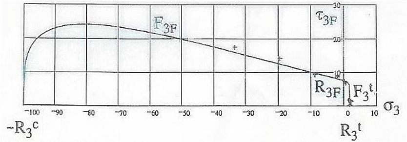
Fig. 22: Failure envelope \sigma_W(\sigma_F) ,C/SiC tube, RT, m=3 , (test data from dissertation B. Thielicke, 1997) {Thi97[
