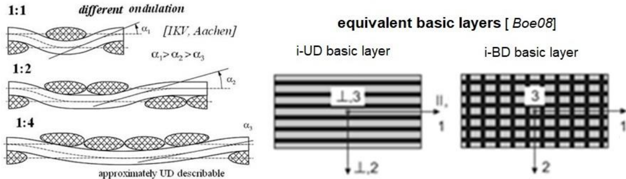
Fig.13: 2D-Modelling of differently woven fabrics with basic layers
