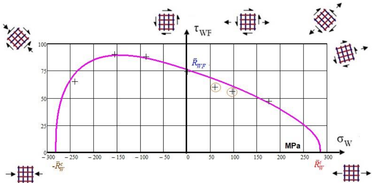
Fig. 20: Off-axis coupon tests, \begin{bmatrix} 0 \\ 90 \end{bmatrix}_S Failure envelope \tau_{WF}(\sigma_W) . (data set Siemens AG). m = 2.6
