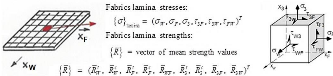
Fig.14: Properties and stresses of the fabric material [Cun98]
