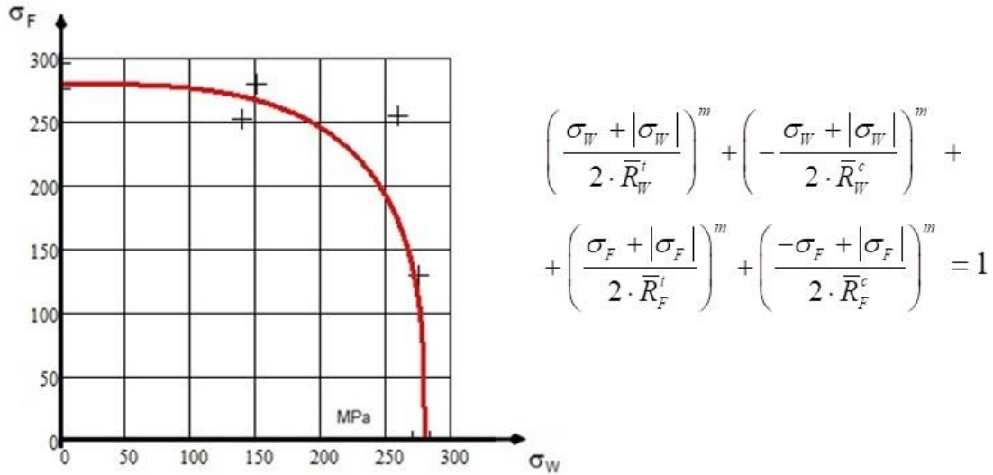
Fig.19: Failure envelope \sigma_W(\sigma_F) . plain weave fabric C/SiC tube for X38 Body Flap, reentry, \sigma_W(\sigma_F) , RT, MAN-Technologie, m=3 , 1997, \bar{R}_W^t \cong \bar{R}_F^t = 278 MPa, CVI process [Cun98, Cun98b]
