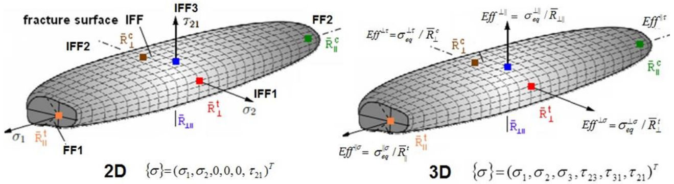
Fig.12: lamina stresses-based surface or fracture body of the UD material and strength-normalized 3D fracture surface [Cun23a, Cun13]
