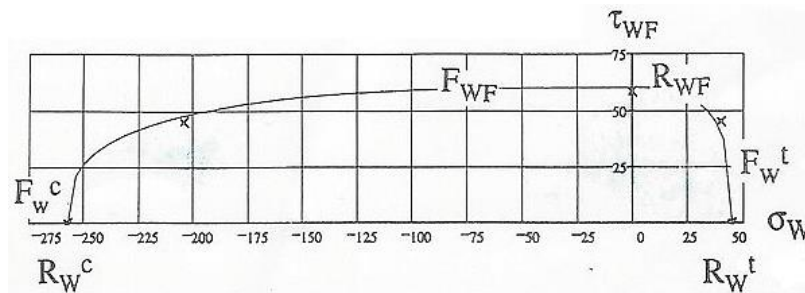
Fig. 21: Failure envelope \tau_{WF}(\sigma_W) , C/C-SiC tube, T=1600^\circ\text{C} , m=3 [Gei97].
