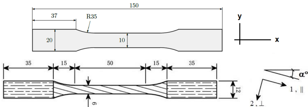
Fig.4, front views: (up) Dogbone-shaped test specimen after ASTM- or EU-standard. Structural coordinate system (CoS , x , y) and material coordinate system (CoS fabric F, W and CoS UD 1 \equiv \parallel , 2 \equiv \perp ). (down) 10°-tensile test specimen (Chamis-Sinclair proposal 1977)
