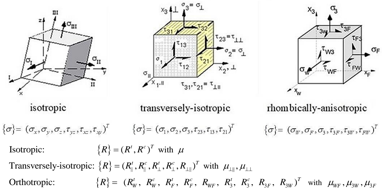
Fig.1: 3D-stress states and strengths employed in ceramic analyses Warp (W, Kette), Fill (F, Schuss, weft). Rhombically-anisotropic = orthotropic. t = tension, c = compression
