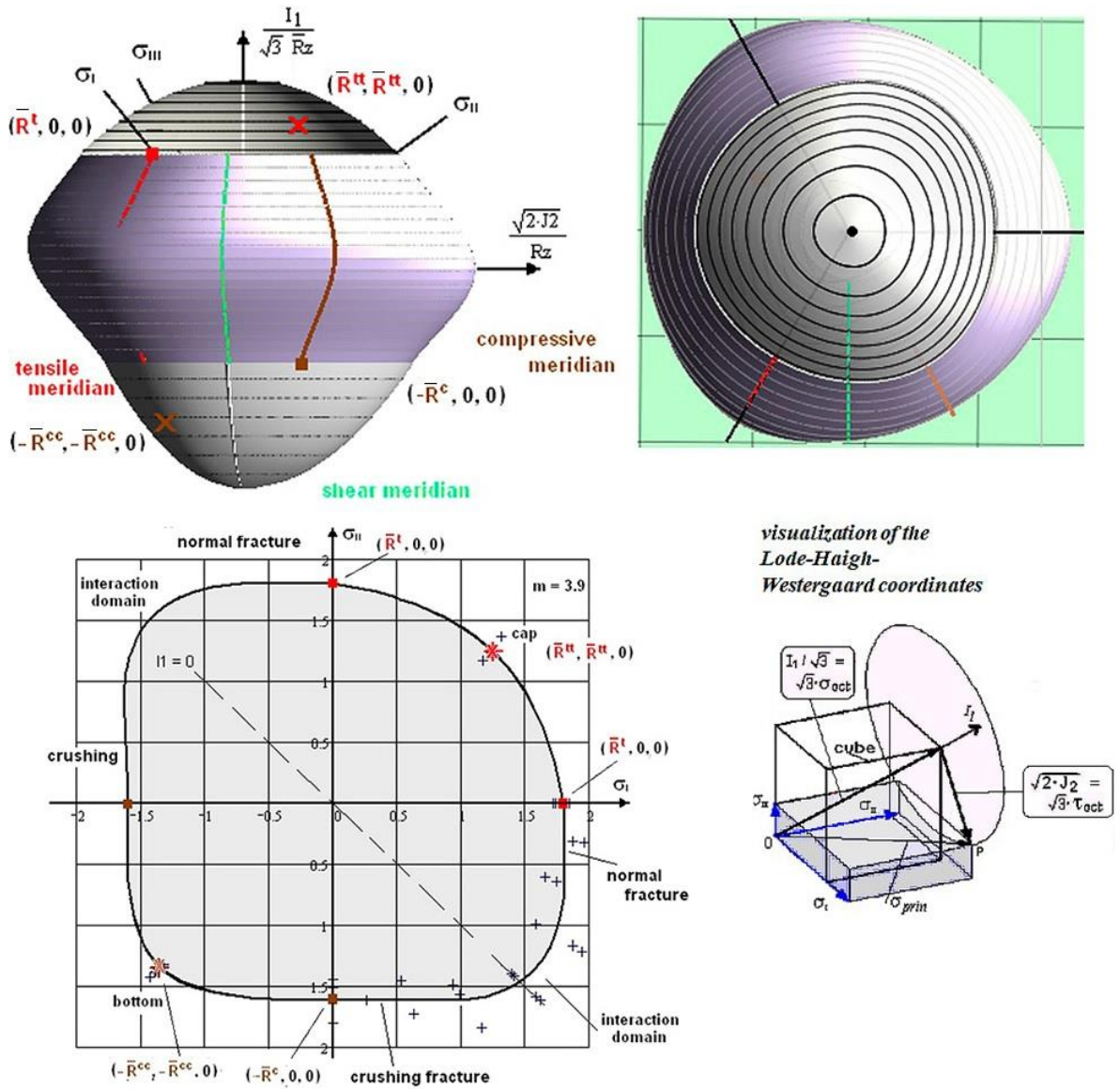
Fig.11, Rohacell 71 IG: Fracture body with its different meridians (left) and view from top (right). The test points are located at a distinct Lode angle of its associated ring \sigma , 120^\circ -symmetry. Foam Rohacell 71 IG: Mapping of 2D-test data in the Principal Stress Plane. MathCad plot [test data: courtesy V. Kolupaev, LBF Darmstadt]
