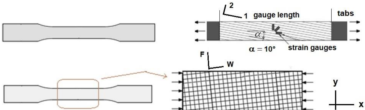
Fig. 5 Typical dogbone coupon test specimens:(up) Off-axis coupon tensile UD test specimen, (down) the shorter \begin{bmatrix} 0 \\ 90 \end{bmatrix}_S fabric plies-composed coupon compression test specimen
